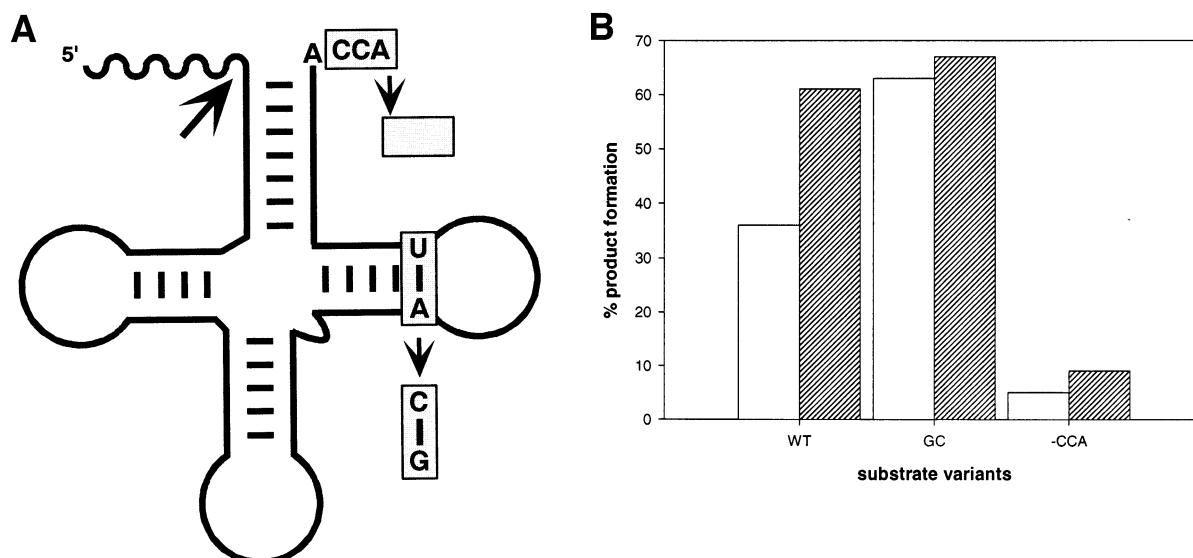
Fig. 3. A: Schematic representation of pre-tRNA Glu mutants. The deletion of the 3' terminal CCA and the changes in the T-stem are indicated by boxes. The 5' flank is drawn as a wavy line and the position of the phosphodiester bond cleaved in the RNase P reaction is shown by a large arrowhead. B: Influence of substrate structure on pre-tRNA cleavage by P. hollandica RNase P RNA. Cleavage of wild type pre-tRNA Glu (WT; A53-U61), the G53-C61 mutant (GC), or the CCA deletion mutant (–CCA) was measured after 30 min (white bars) or 60 min (hatched bars).
